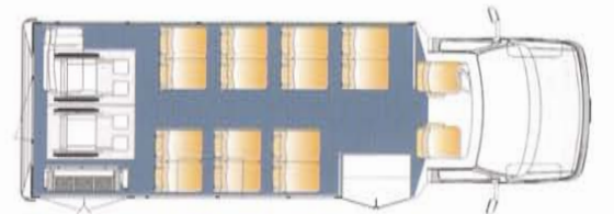
15 Passenger Plus 2 Wheelchair Positions Plus Foldaway
